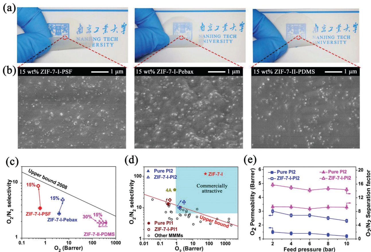
Fig. 4 (a) The physical appearance, (b) SEM images of cross-sections, (c) pure component O_2 and N_2 permeation properties measured at 2 bar upstream pressure and 35\text{ }^\circ\text{C} , and (d) comparison of O_2/N_2 separation performance in this work with the other MMMs. The commercially attractive region was identified by Koros and co-workers. 52 (e) O_2/N_2 (50 : 50) mixed-gas permeation results as a function of feed pressure on the pristine 6FDA/BPDA-ODA (PI2) films and 15 wt% ZIF-7-I-PI2 membranes. The total feed pressure and permeating temperature are 4 bar and 35\text{ }^\circ\text{C} , respectively. Closed and open symbols represent the results of pristine PI2 film and 15% ZIF-7-I-PI2 membranes, respectively.
