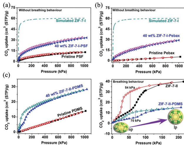
Fig. 3 \text{CO}_2 adsorption properties of pristine polymer, ZIF-7 nanocrystals and 40 wt% ZIF-7-polymer composites derived from (a) PSF, (b) Pebax ® 1657 and (c) PDMS. Closed and open symbols represent adsorption and desorption branches, respectively. The dashed line is the GCMC adsorption of the ZIF-7-I phase. ZIF-7-II-PDMS composite can be reversibly transformed from a narrow pore (type-II) to a large pore (type-I) phase. The \text{CO}_2 uptake for all samples was assessed in the high-pressure region (up to 10 bar) by analysis of the respective isotherms measured at 308 K.
