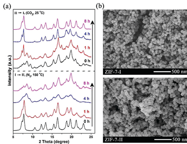
Fig. 1 (a) XRD patterns and (b) SEM images of as-synthesized ZIF-7-I and ZIF-7-II nanocrystals. The phase transition from ZIF-7-I to ZIF-7-II structure was conducted at 150 °C with the purge of N 2 , while phase transition from ZIF-7-II to ZIF-7-I was performed at 25 °C with the purge of pure CO 2 .
