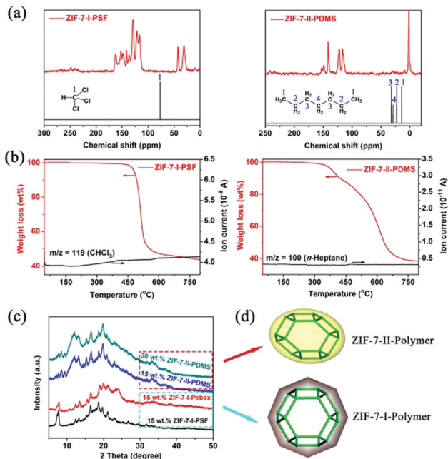
Fig. 2 (a) Solid-state ^{13}\text{C} CP-MAS NMR spectra, (b) TGA and ion current trace curves, (c) XRD patterns and (d) structural schematic diagram of ZIF-7-polymer composites derived from three commercial polymers.
