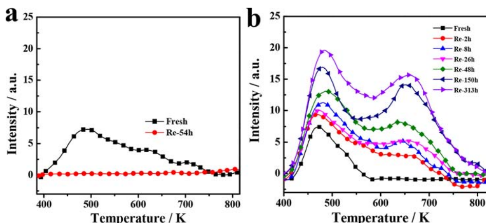
Figure 4. \text{NH}_3 -TPD profiles of fresh samples and regenerated samples after various reaction time: (a) \text{AlCl}_3/\text{F-Silicate-1} and (b) \text{AlCl}_3/\text{Silicate-1} .
