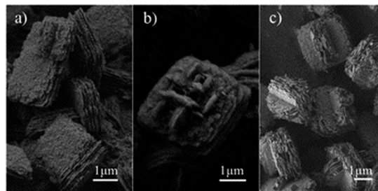
Fig. 19 SEM images of hierarchical SAPO-34 synthesized for (a) 6 h, (b) 10 h and (c) 20 h, showing the preferential growth changing from one orientation to three orientations. Reproduced from ref. 135 with permission from The Royal Society of Chemistry. 135
