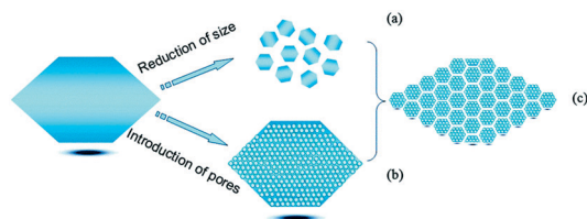
Fig. 4 The strategies to shorten the diffusion path length and increase the external surface area: (a) downsizing the crystals, (b) introduction of additional pores and (c) decrease of size and introduction of auxiliary pores in nanosized crystals. Reproduced from ref. 16 with permission from The Royal Society of Chemistry. 16
